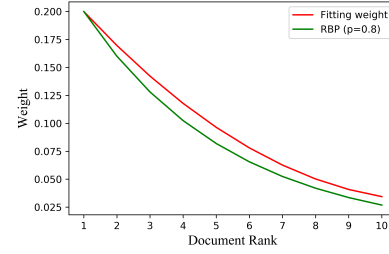
Figure 2: Comparison of document weight between our fitted model and RBP ( p=0.8 ).
