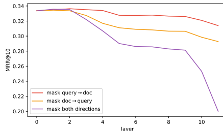
Figure 4: Ranking performance of Query-Doc Interaction Mask Experiment.
