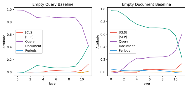
Figure 2: Attribution on different layers
