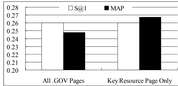
Figure 2 Retrieval performances in the measure of success rate at 1 st document and mean average precision.
